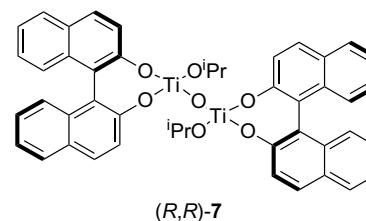
Figure 2. \mu -Oxo bis(binaphthoxy)(isopropoxy)titanium complex ( R,R )-7 developed by Maruoka and co-workers. 40
