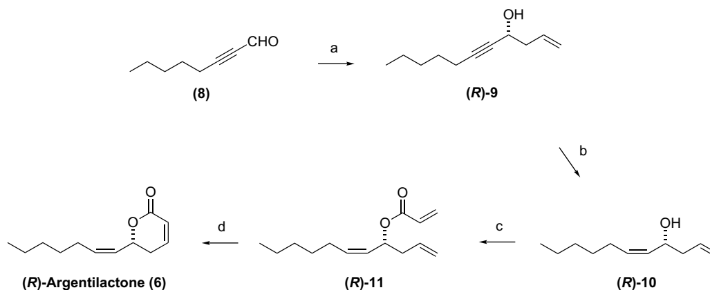
Scheme 1. (a) ( R )-BINOL (10 mol%), \text{Ti}(\text{O}i\text{Pr})_4 (15 mol%), \text{TiCl}_4 (5 mol%), \text{Ag}_2\text{O} (10 mol%), allyltributyltin (1.1 equiv), \text{CH}_2\text{Cl}_2 , -20^\circ\text{C} , 24 h (89%; 84% ee); (b) quinoline (2.0 equiv), Lindlar catalyst (10 mol%), \text{EtOAc} –1-octene (1:1) (74%); (c) acryloyl chloride (1.8 equiv), \text{Et}_3\text{N} (3.6 equiv), \text{CH}_2\text{Cl}_2 , 0^\circ\text{C} (86%); (d) Grubbs' catalyst [ (\text{PCy}_3)_2\text{Cl}_2\text{Ru}=\text{CHPh} ] (10 mol%), \text{CH}_2\text{Cl}_2 (70%).
